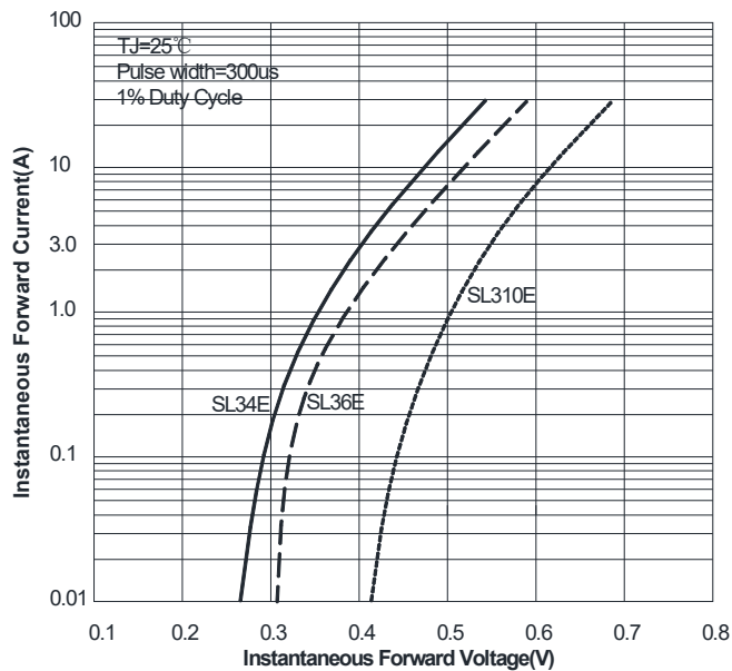
FIG3: Forward Voltage
